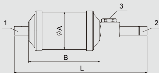
① Inlet
