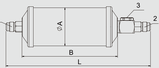
③ Sight Glass
